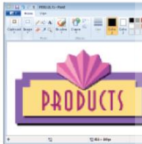
FIGURE 6-26 Graphics software.
